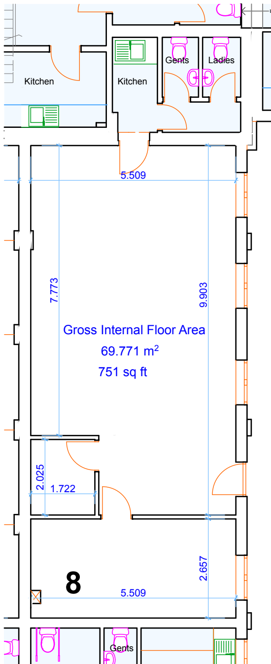
0. Ground Floor 1:100
